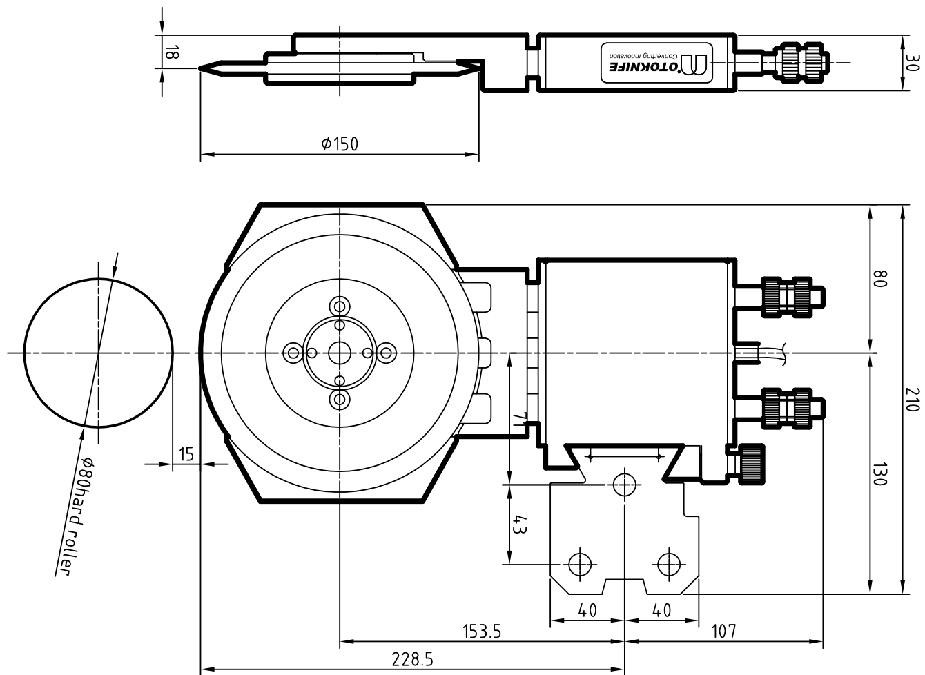
MT-A510 Heavyduty Type Slitting Score Air Knife
