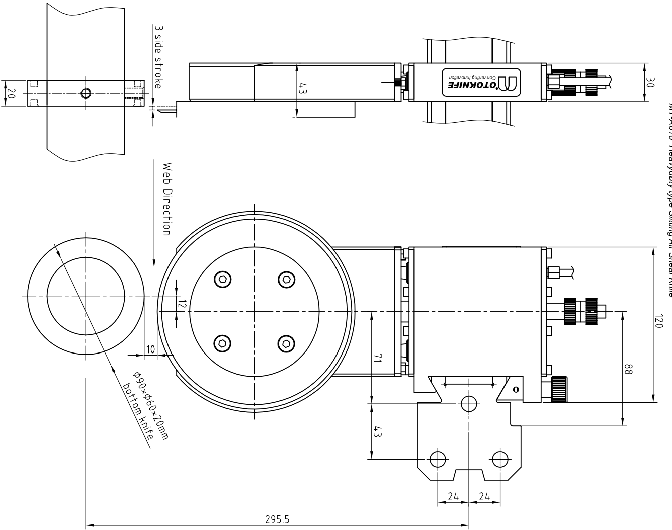
MT-A610 Heavyduty type Slitting Air Shear Knife
